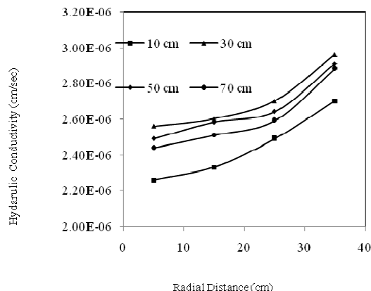
Figure 8: Variation of hydraulic conductivity with radial distance on 365 days curing
