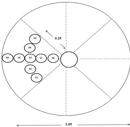
Figure 2. Plan of the test tank showing locations for collection of leachate samples
