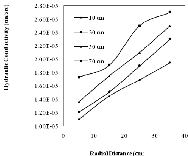
Figure 7: Variation of hydraulic conductivity with radial distance on 180 days curing
